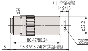
LCD Plan Apo NUV 50× (t0.7)
