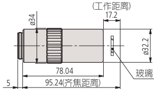
LCD Plan Apo NUV 20× (t0.7)
